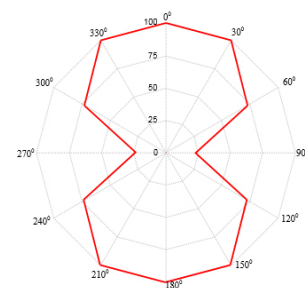
Read range (%) at various angle
