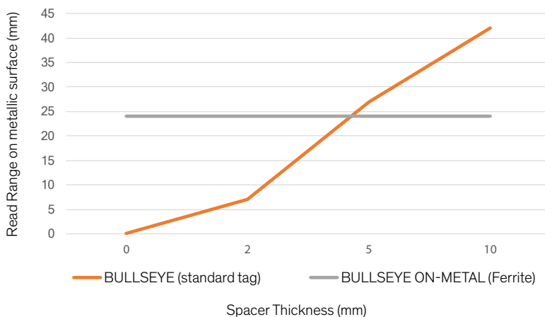
Comparison standard inlays with spacer and inlays with ferrite material
